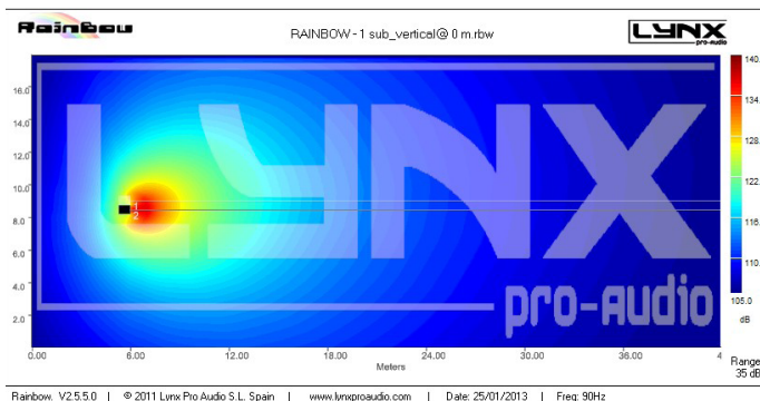
SPL MAP of LYNX LX-218S - Vertical view
